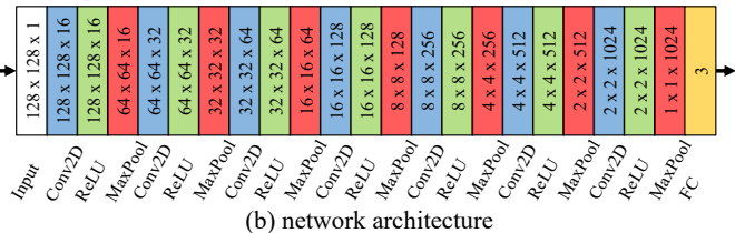
(b) network architecture
